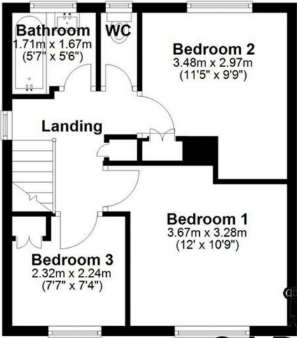
First Floor Approx. 36.1 sq. metres (389.0 sq. feet)
