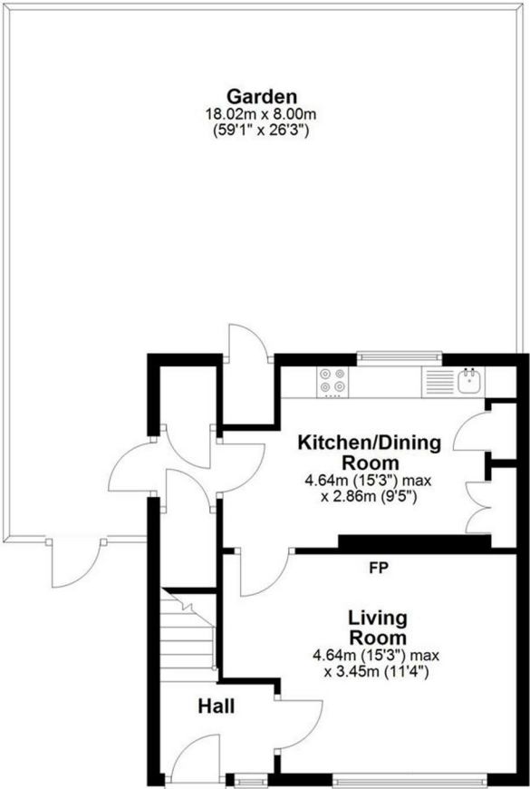
Ground Floor Approx. 36.1 sq. metres (388.4 sq. feet)
